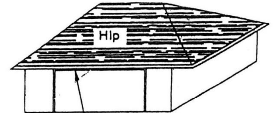
Lintel over door opening Supporting roof loads
