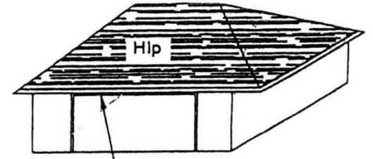
Lintel over door opening Supporting roof loads
